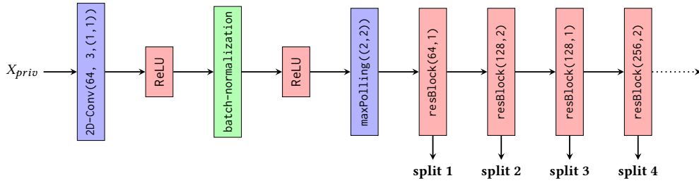
Figure 3: Architecture of the client’s network f divided in 4 different depth levels. The internal setup of the adopted residual blocks is described in Algorithm 2 (Appendix B).
